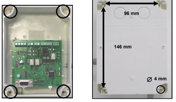
Picture 2 - Wall fixing screw holes, their distances from each other and the maximum allowed screw diameter
