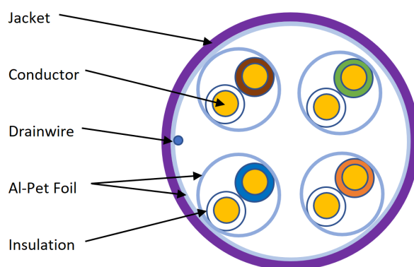
Cross-section diagram
