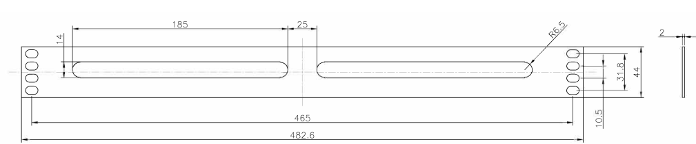
Product drawing (100-610)
